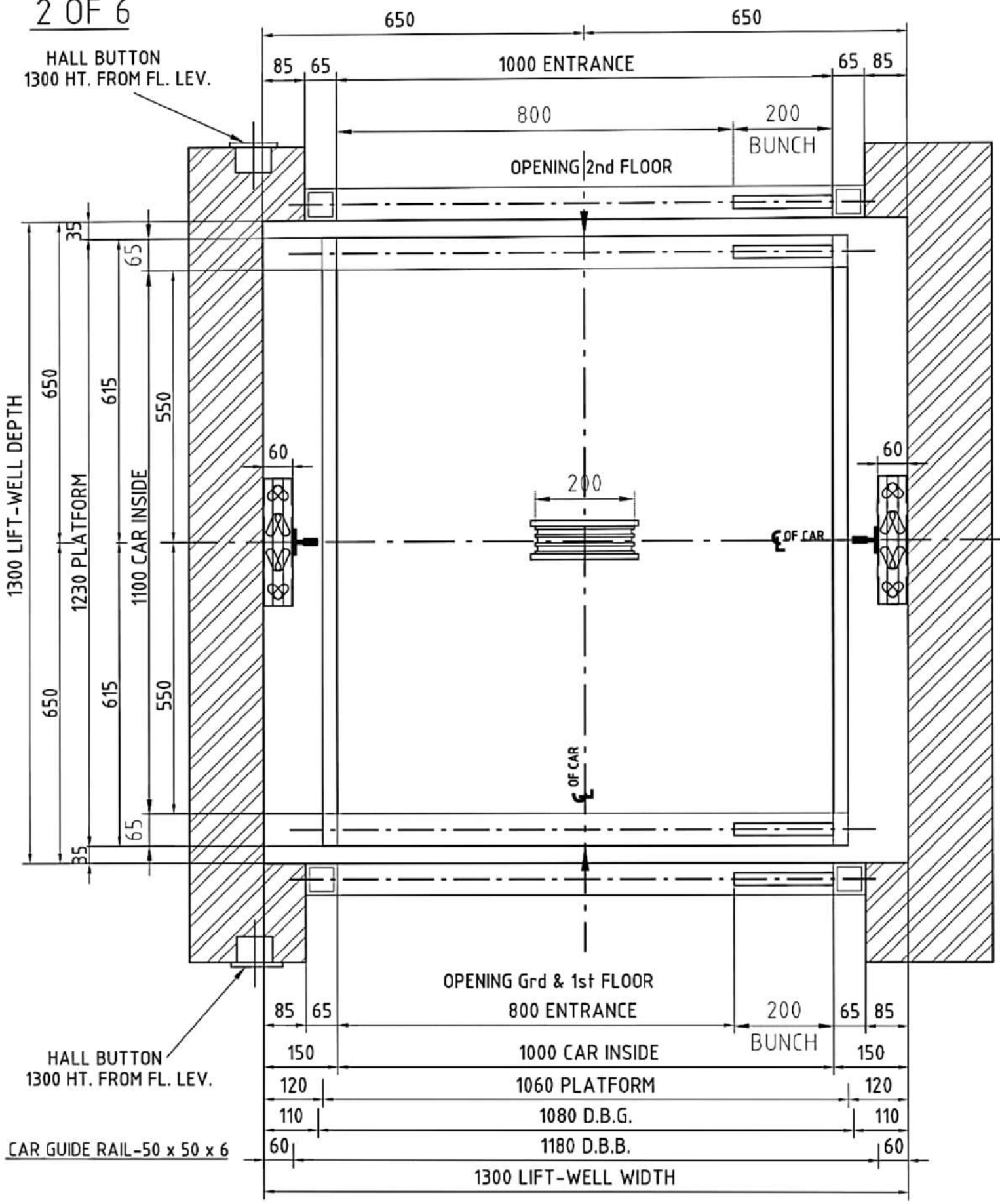
LIFT-WELL PLAN
