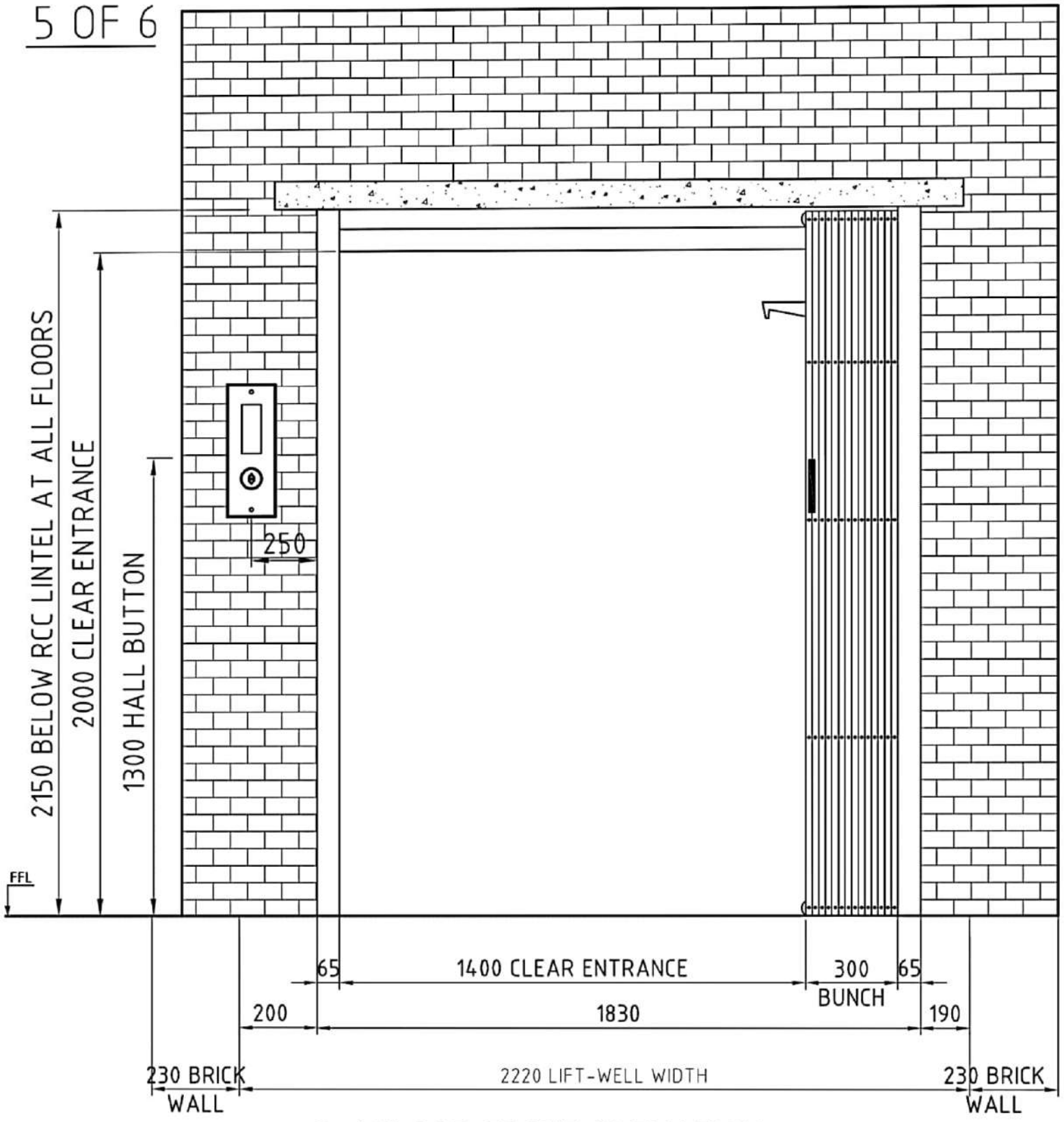
Grd FLOOR FRONT ELEVATION
