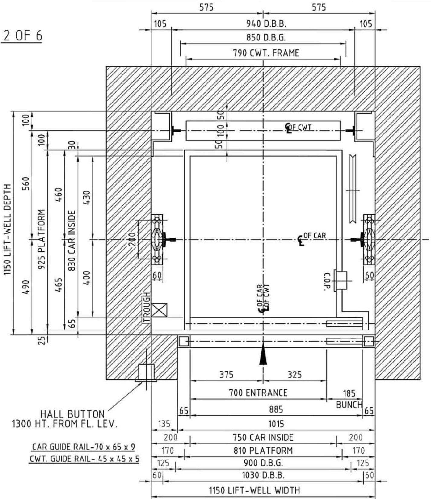
LIFT-WELL PLAN
